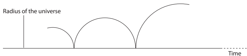
Fig. 3.10: Oscillating Model with entropy increase. Due to the conservation of entropy each successive oscillation has a larger radius and longer expansion time.
